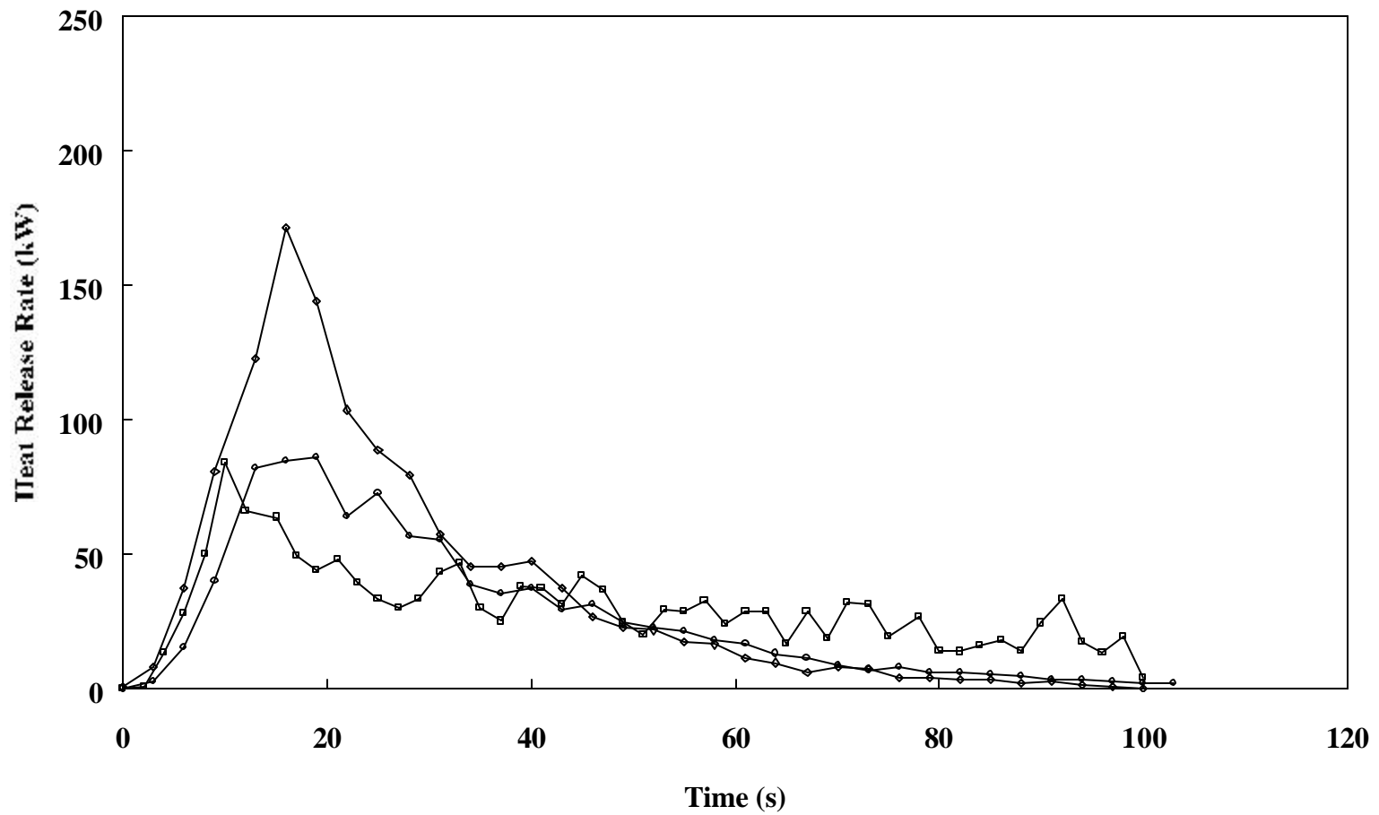
Figure A1. Heat release rates of 250 mL gasoline spill fires on wood parquet floors
